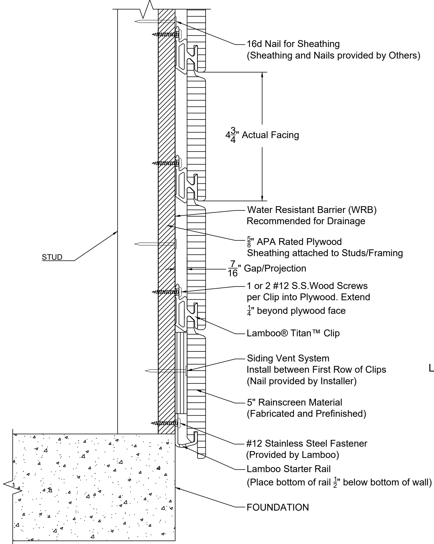
LAMBOO® TITAN™ CLIP - 3 HOLE (MEETS FBC REQUIREMENTS FOR HURRICANE RATED ZONES)
