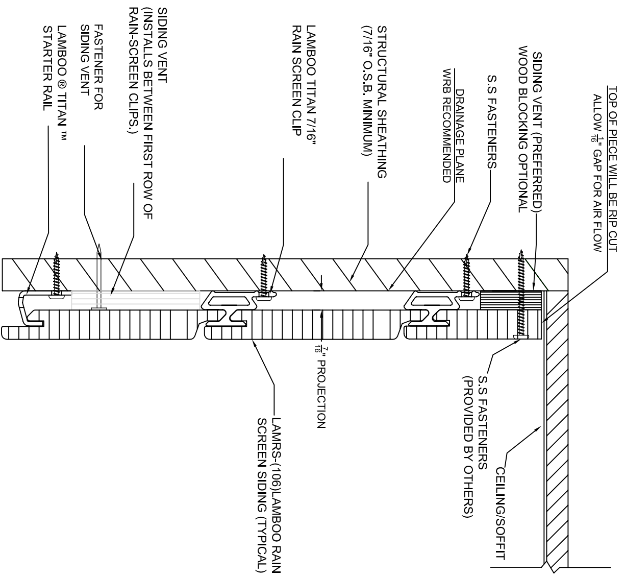
ATTACHMENT DETAIL: WALL TO CEILING ON SHEATHING
